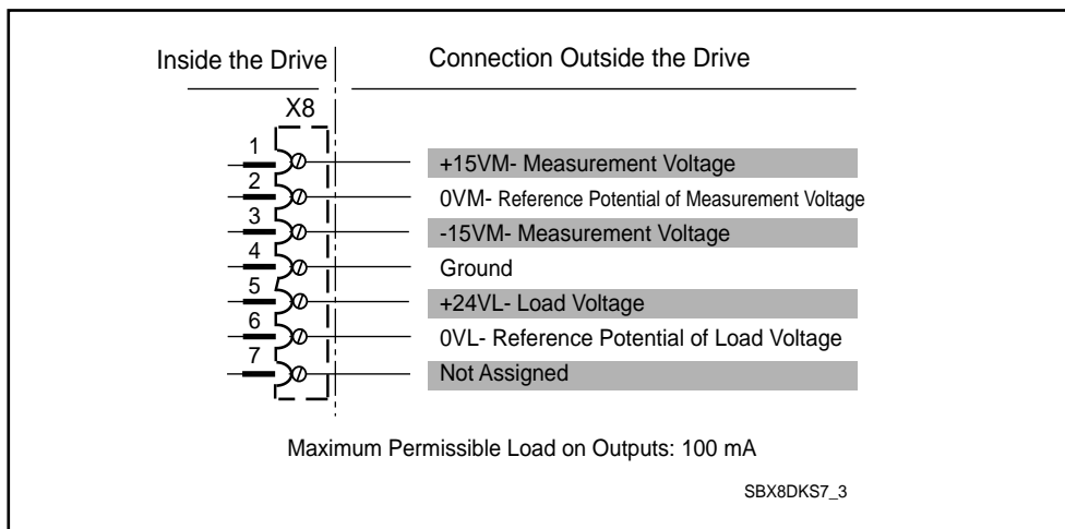
Figure 7.3: Signal voltages at push-in terminal block X8.
